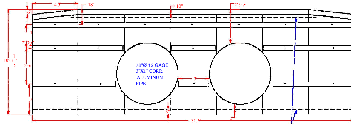
END VIEW- INLET HEADWALL
