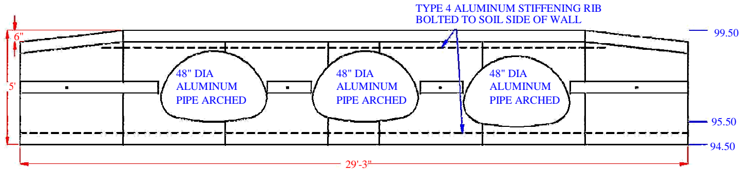
END VIEW- INLET & OUTLET HEADWALL
